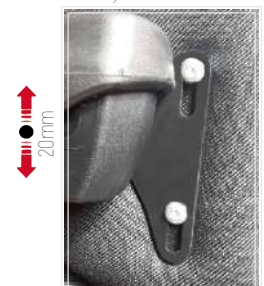
Adjustable Armrest
