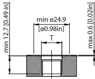
Figure 5: T: 9/16-18 UNF, ISO 11926-1
