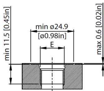
Figure 6: E: M14 x 1.5, ISO 6149-1
