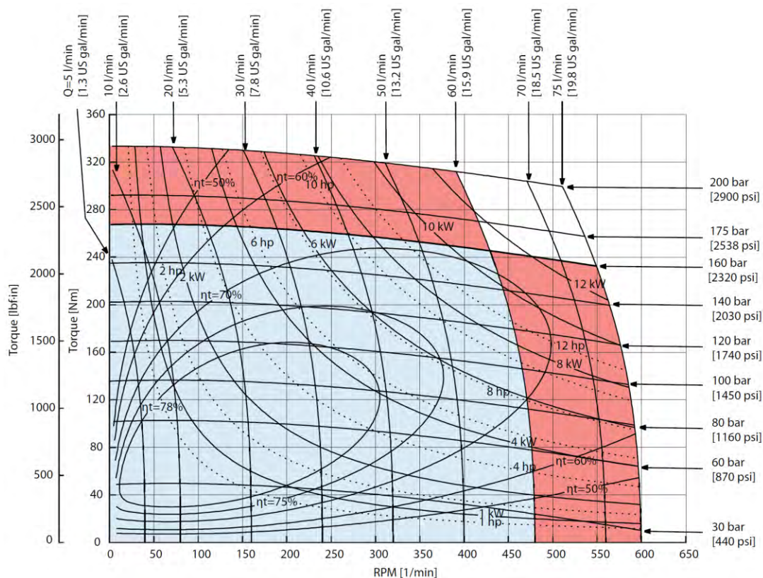
Figure 18 OMP X 125 function diagram
