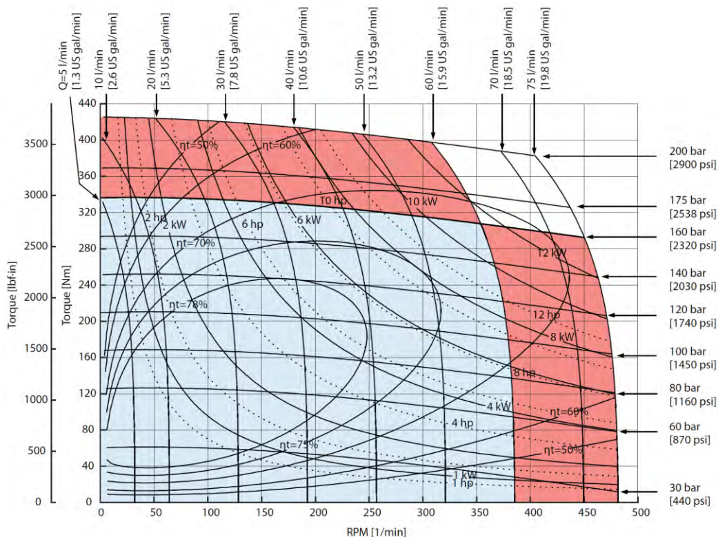
Figure 19 OMP X 160 function diagram
