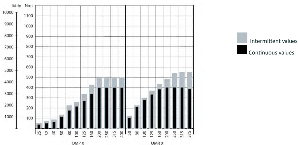
Figure 2 Maximum torque
