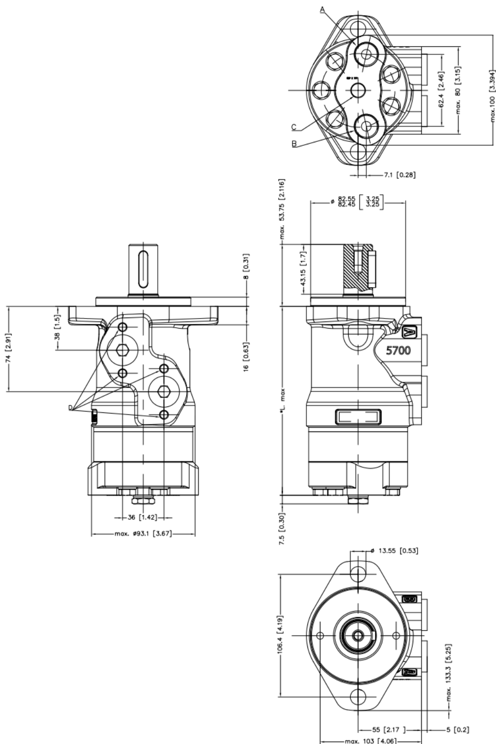
Figure 31 OMP X end port A2-flange EU version
