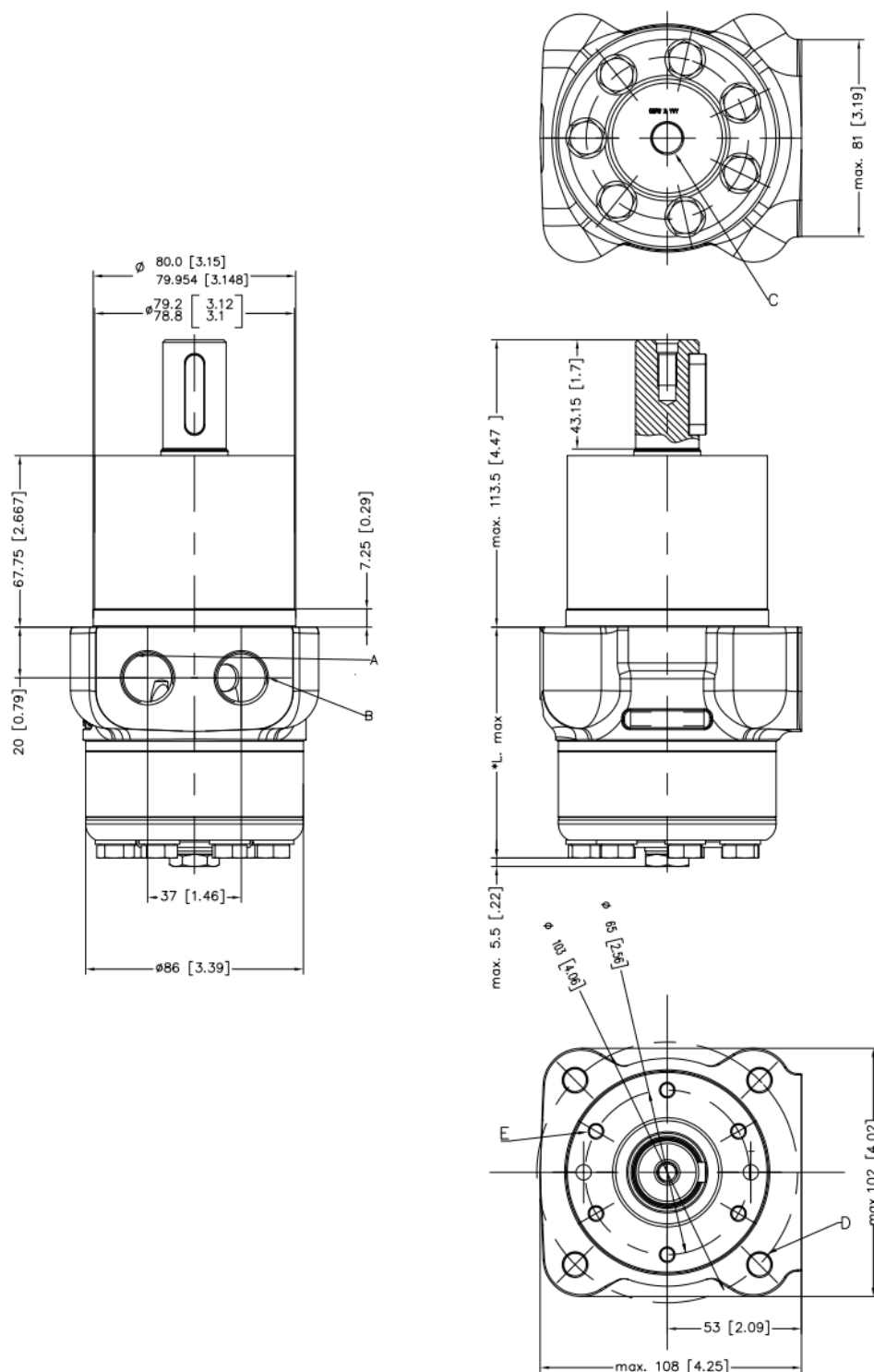
Figure 32 OMPW X and OMPW X N EU version
