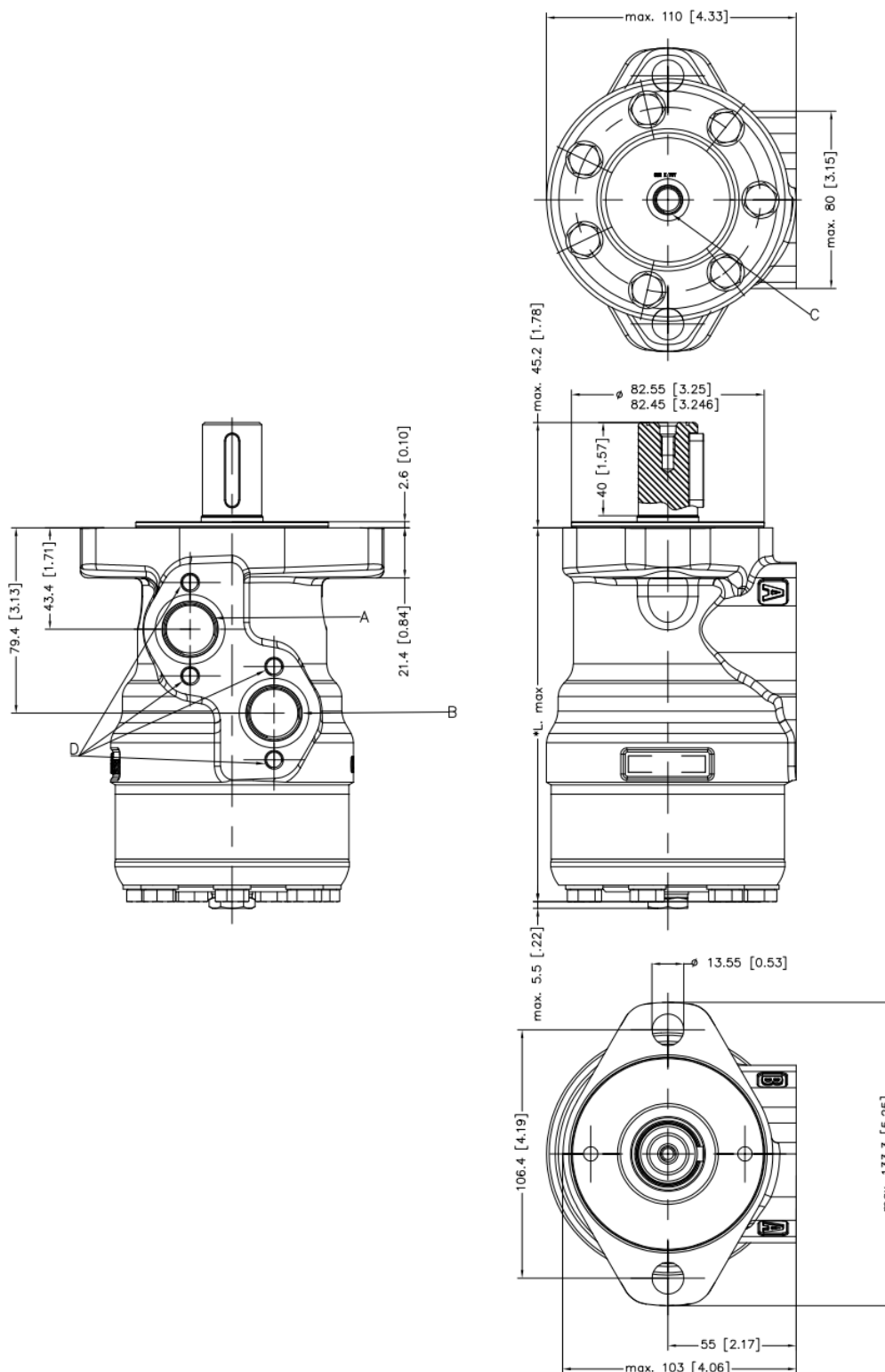
Figure 50 OMR X side port offset (A2-flange) US version
