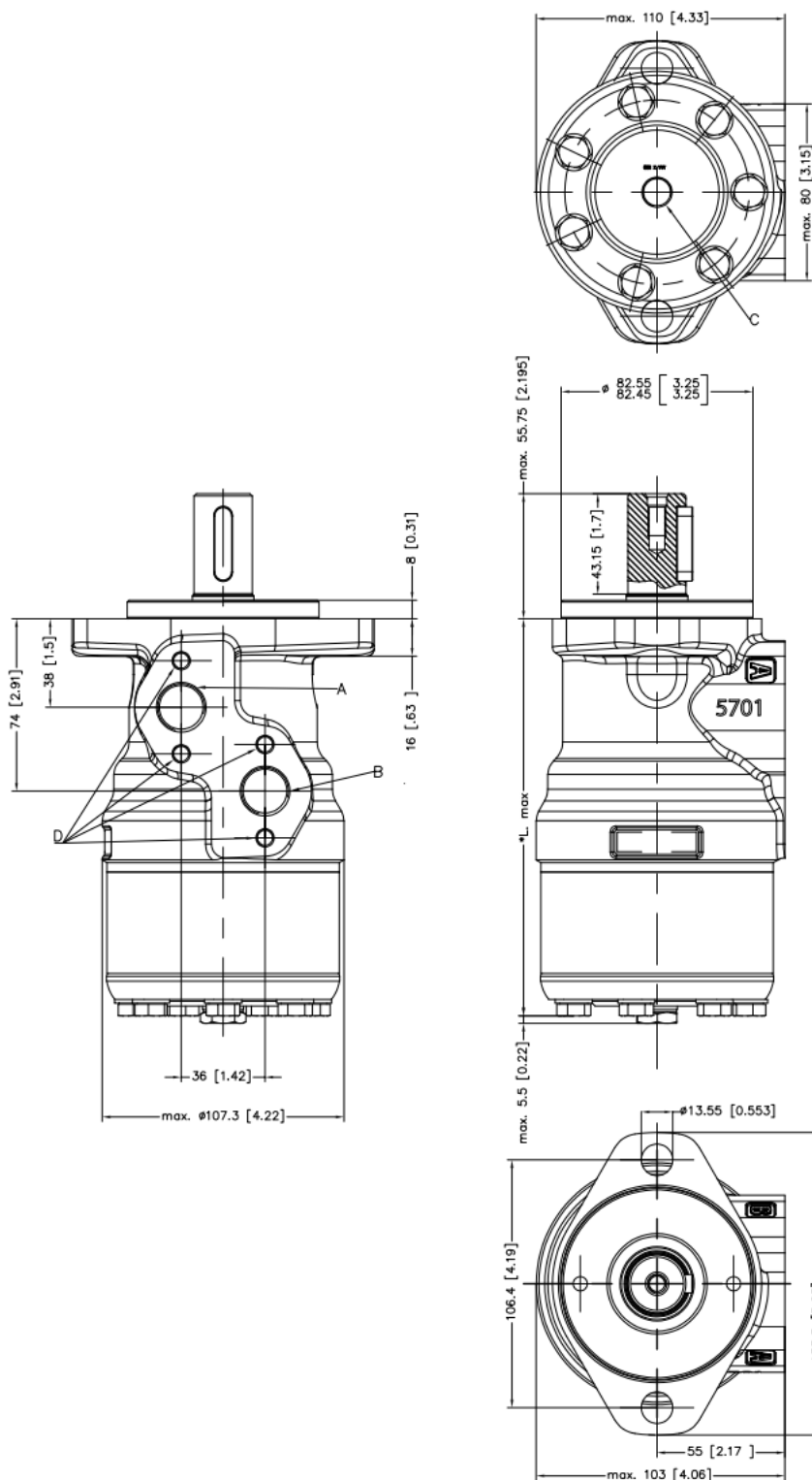
Figure 48 OMR X side port (A2- flange) EU version
