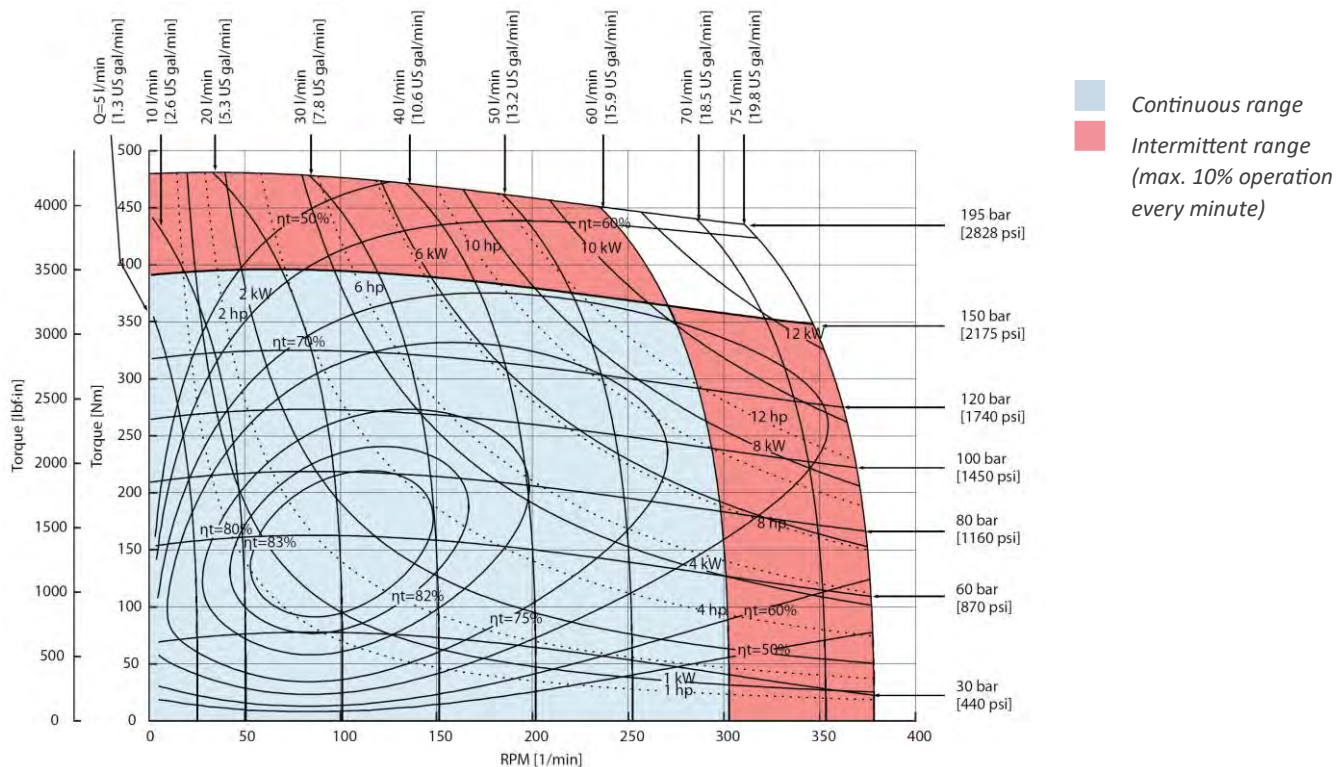
Figure 43 OMR X 200 function diagram
