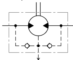
Figure 4 OMP X/ OMR X without drain connection
