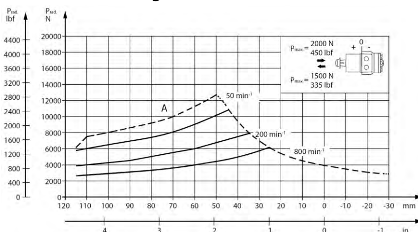
Figure 11 OMPW X with needle bearings shaft loads
