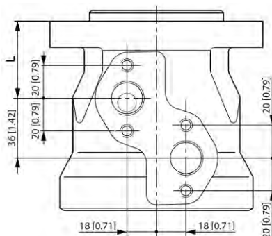
Figure 29 OMP X manifold mount
