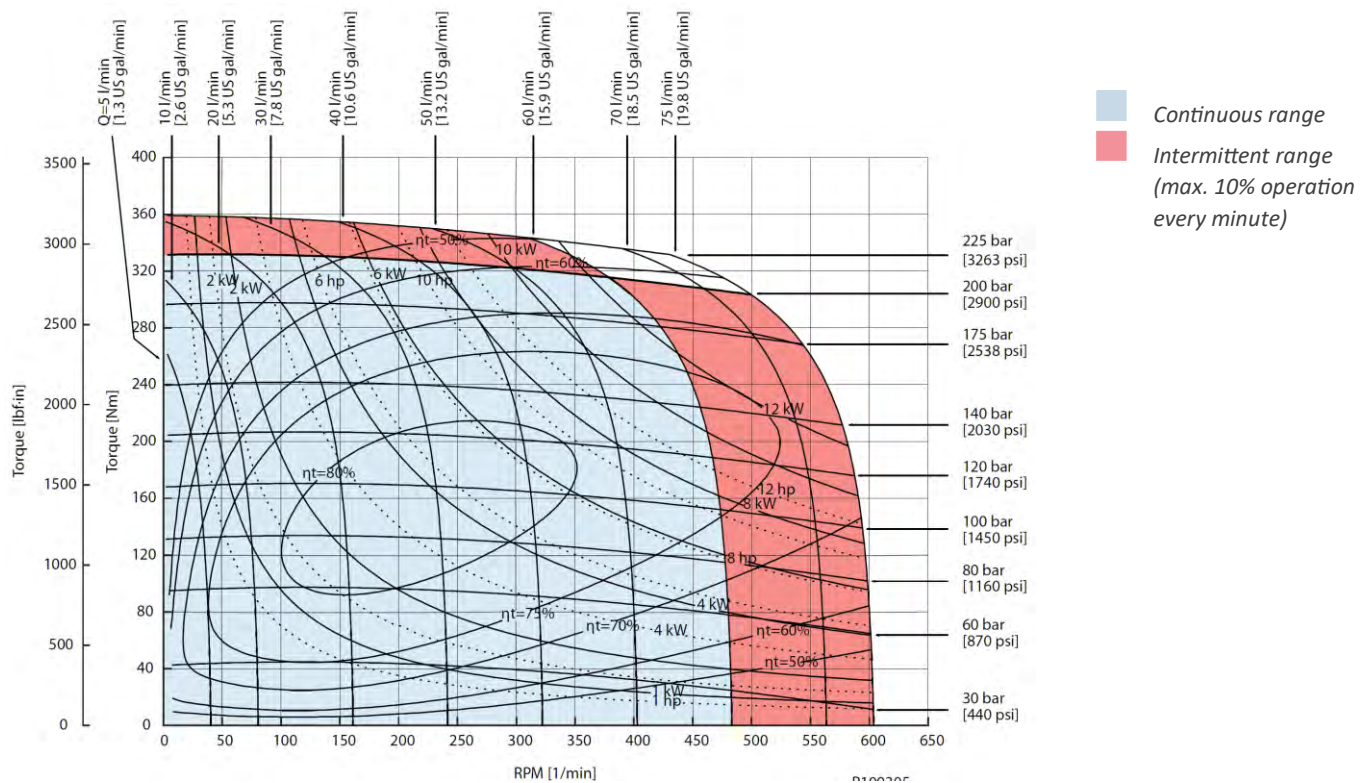
Figure 41 OMR X 125 function diagram
