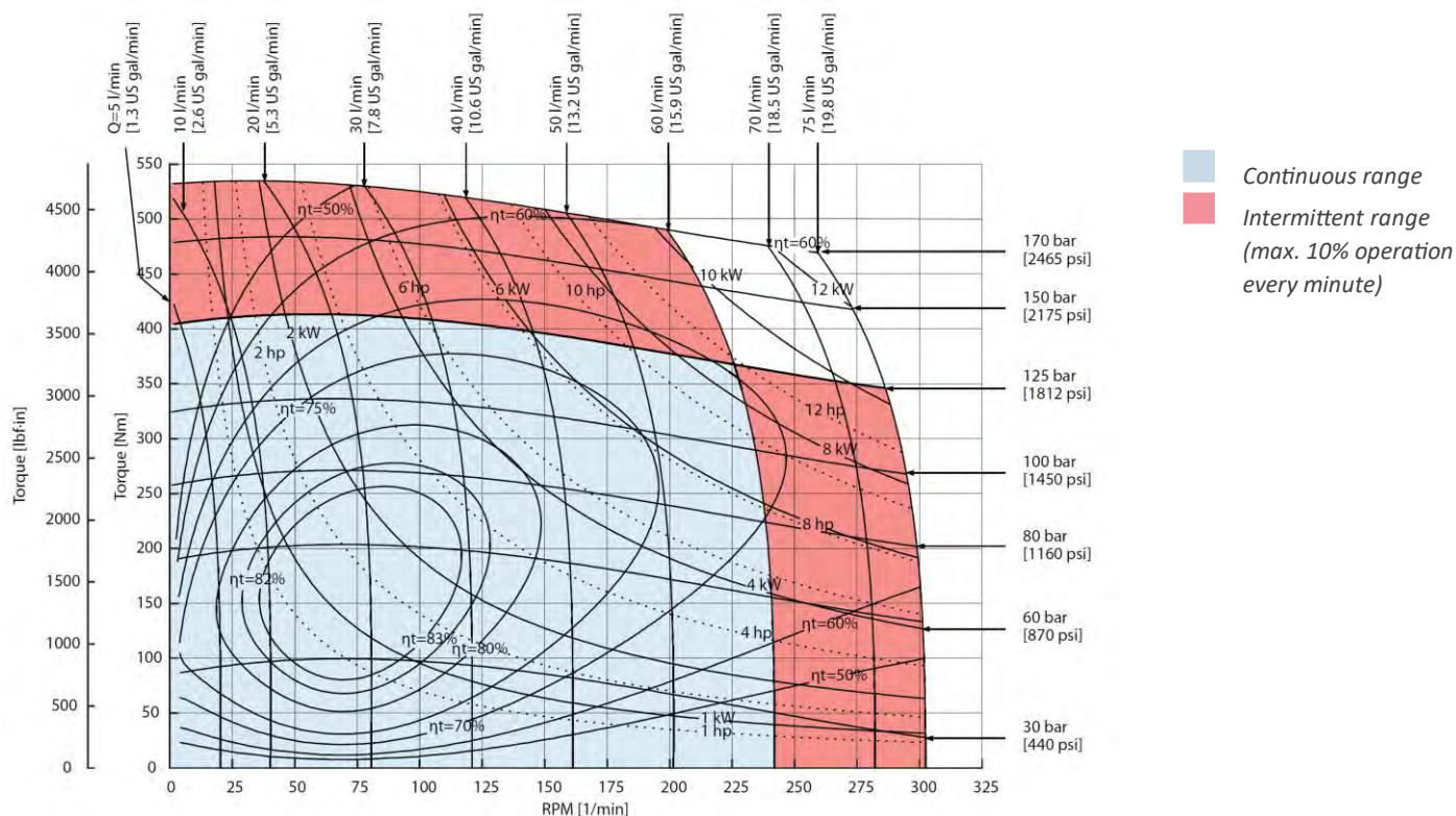
Figure 44 OMR X 250 function diagram
