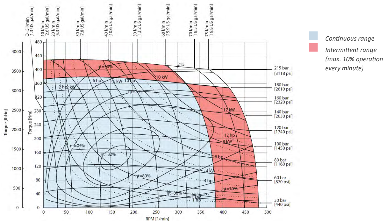
Figure 42 OMR X 160 function diagram
