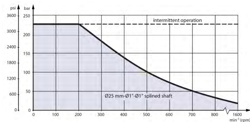
Figure 5 OMP X Maximum permissible shaft seal pressure
