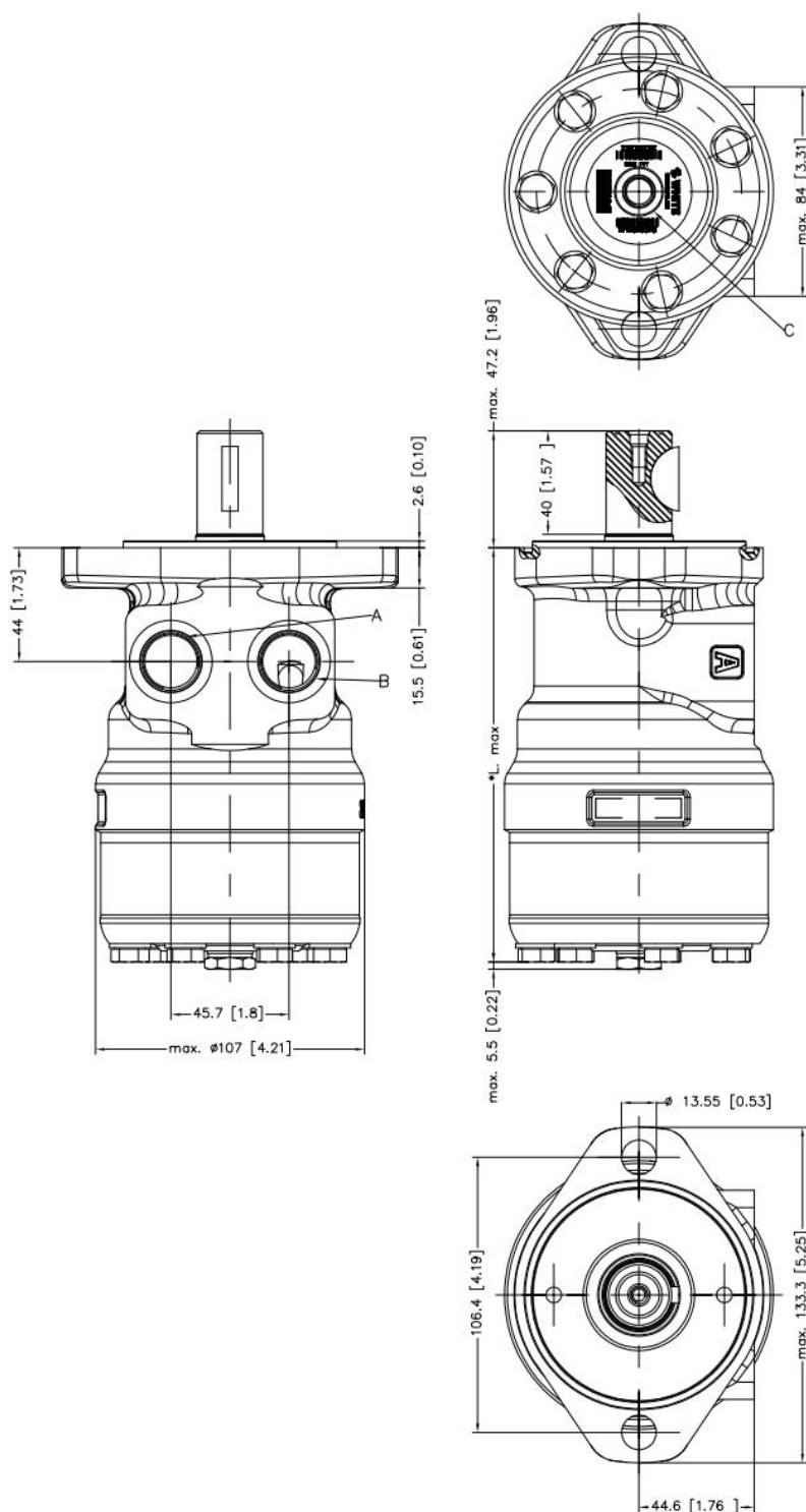
Figure 51 OMR X side port (A2-flange) US version
