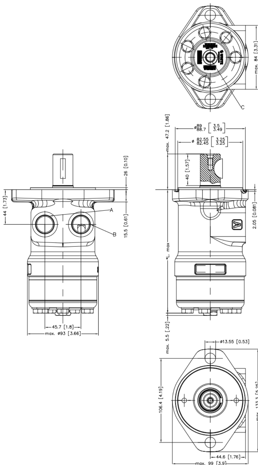
Figure 34 OMP X side port aligned A2- flange (US version)
