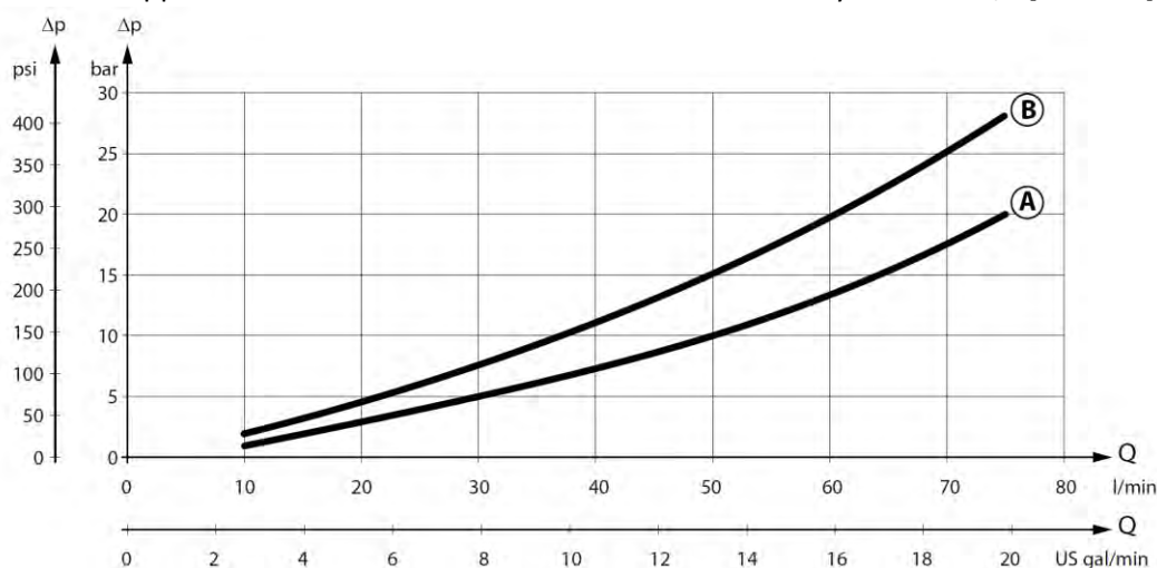
Figure 6 OMP X Motors Pressure drop
