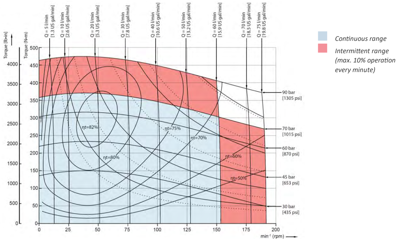
Figure 47 OMR X 400 function diagram
