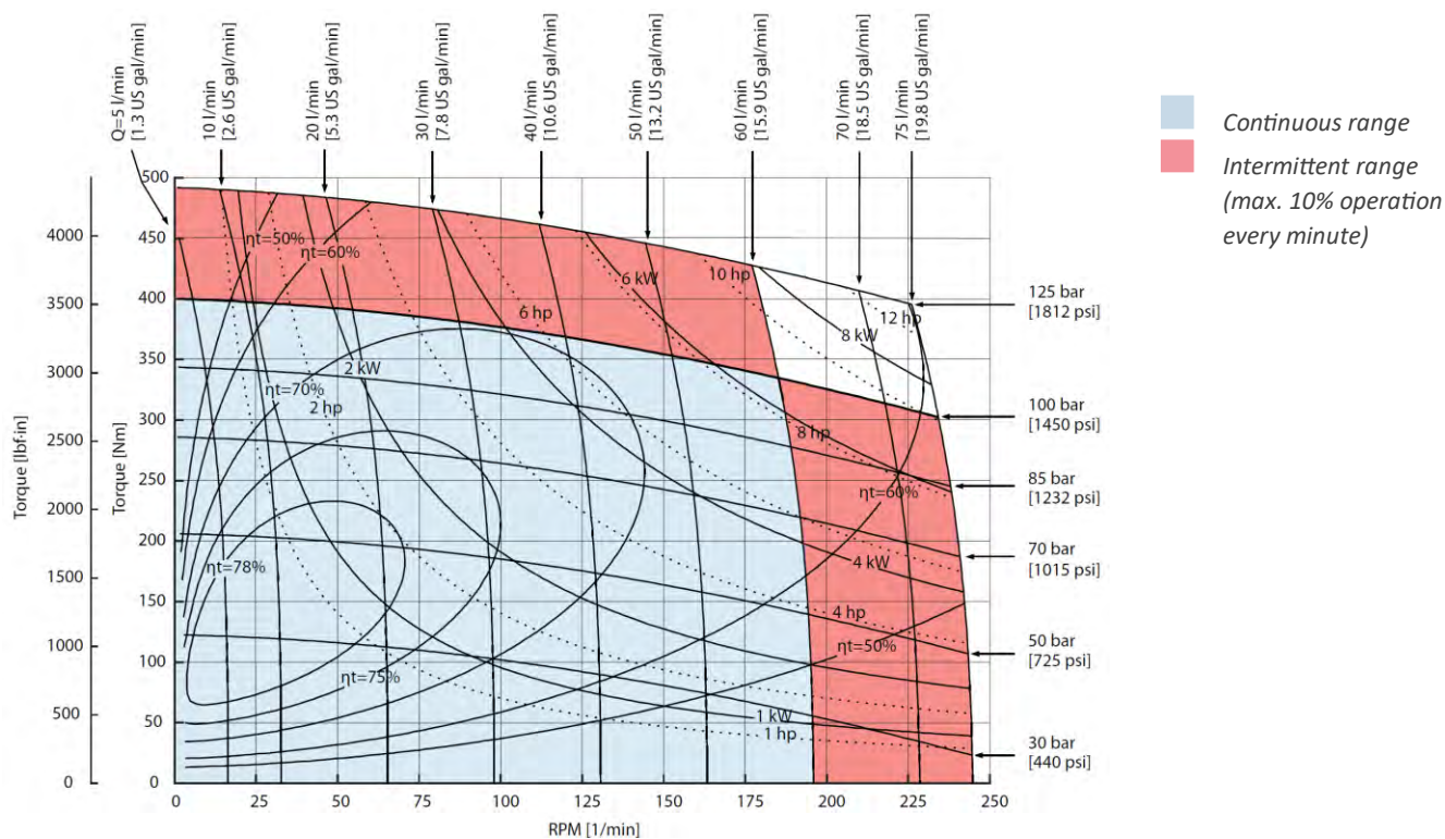
Figure 22 OMP X 315 function diagram
