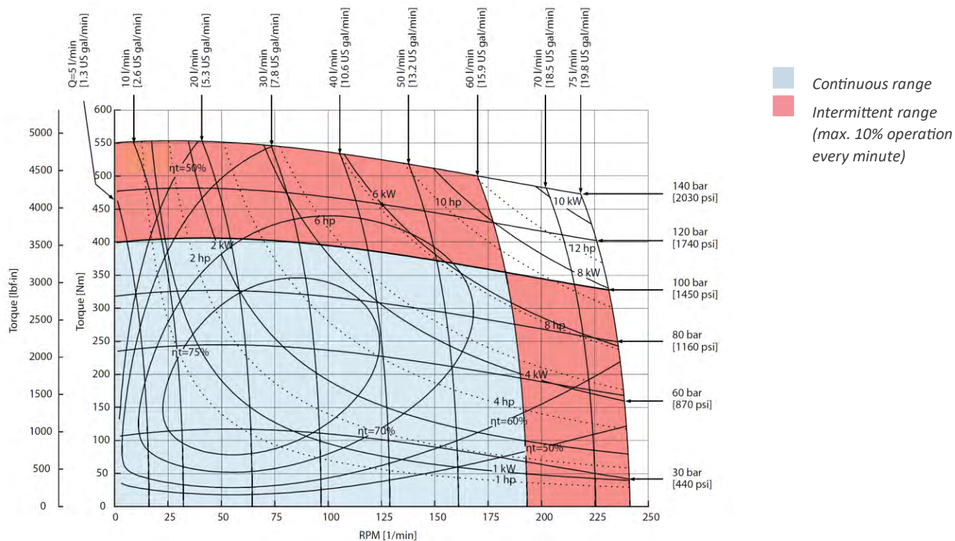
Figure 45 OMR X 315 function diagram
