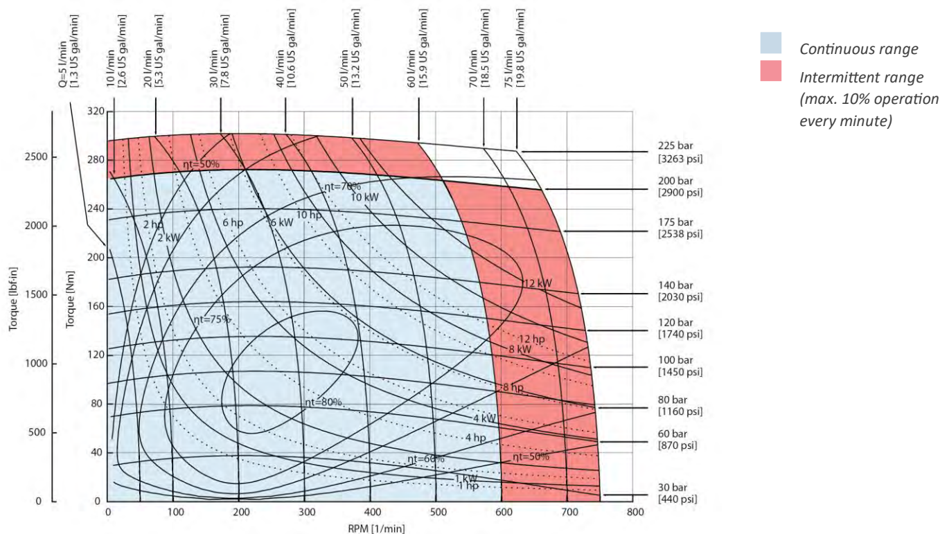
Figure 40 OMR X 100 function diagram
