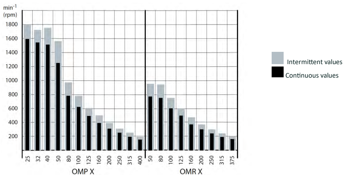
Figure 1 Maximum speed
