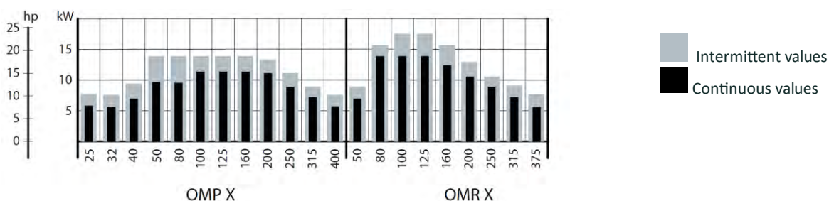
Figure 3 Maximum output
