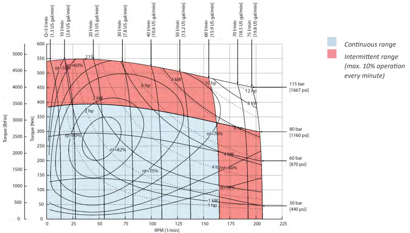
Figure 46 OMR X 375 function diagram
