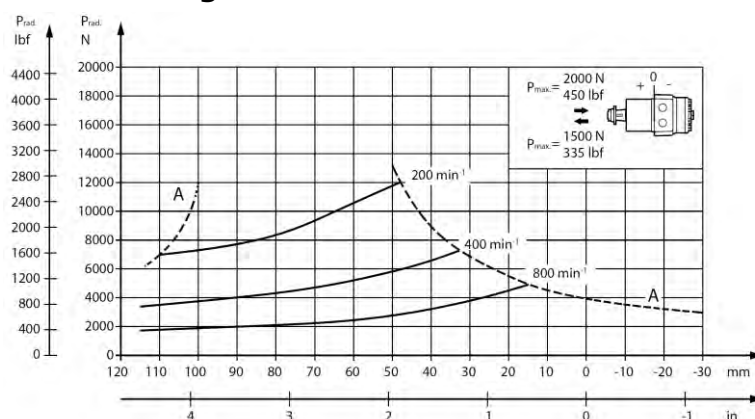
Figure 10 OMPW X with slide bearings shaft loads
