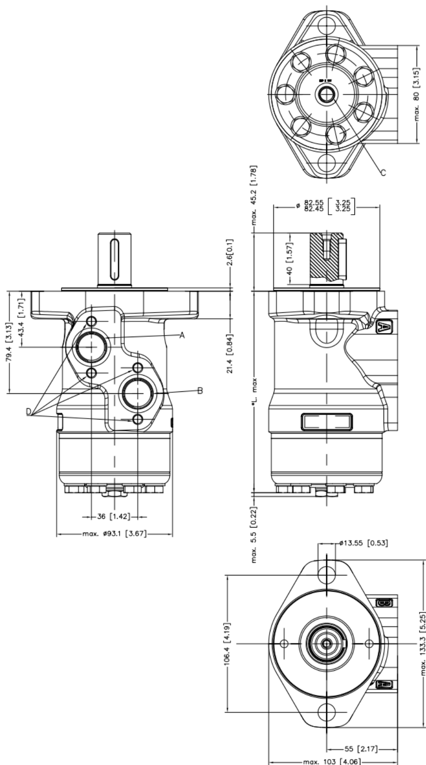
Figure 33 OMP X side port offset A2- flange (US version)
