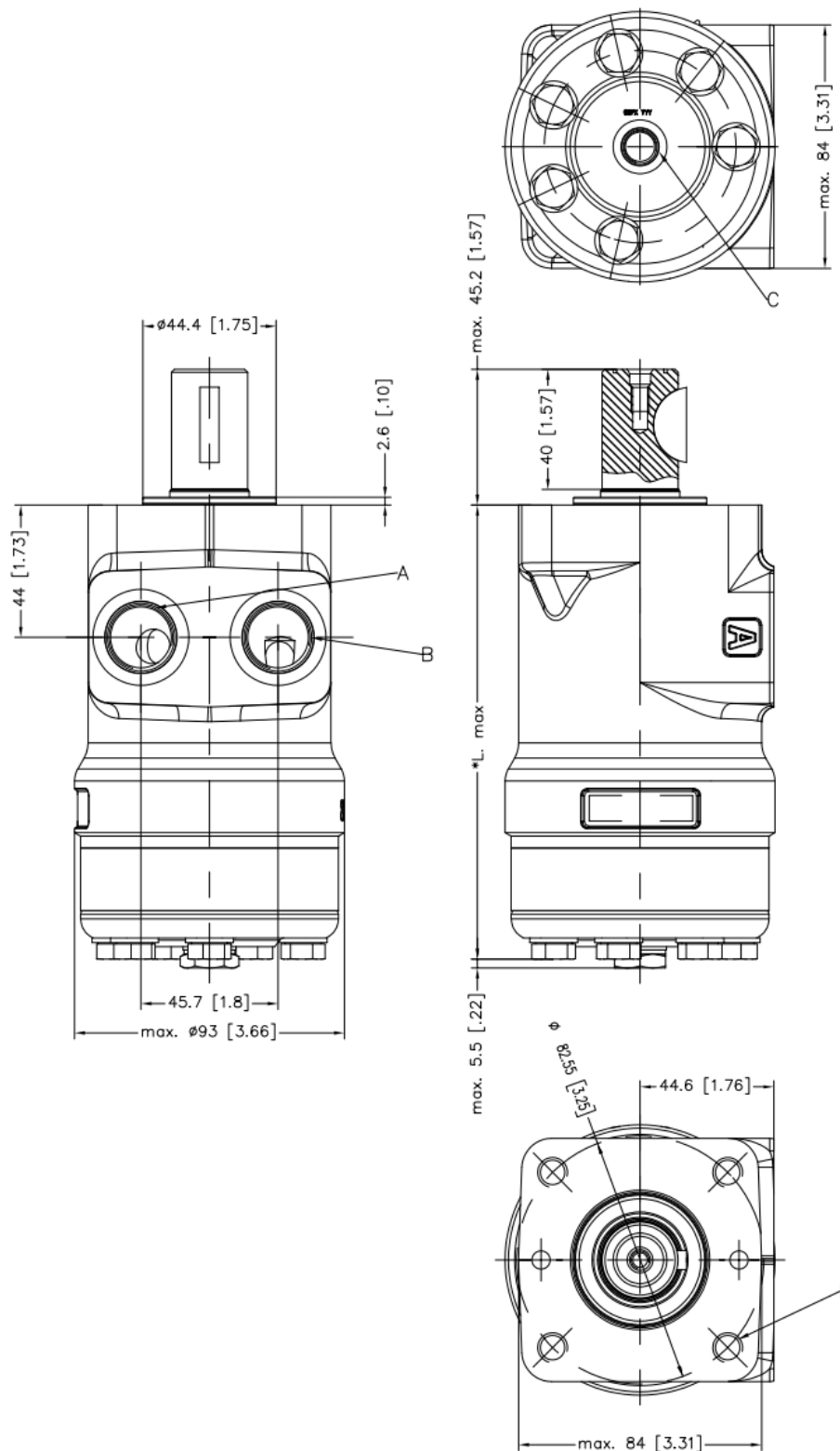
Figure 35 OMP X side port aligned C-flange US version
