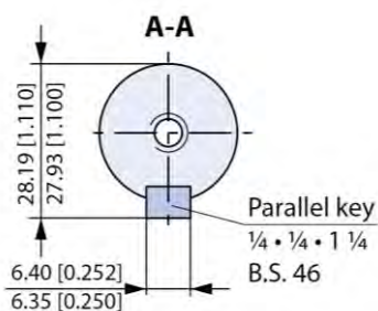
Cylindrical shaft 1 in; Parallel key B.S. 46 (US version)
