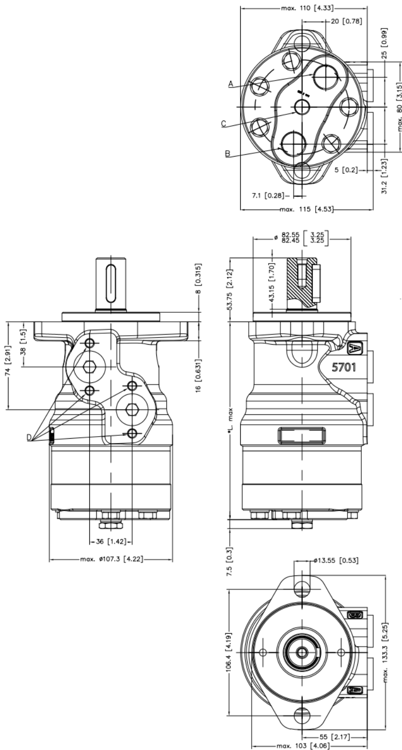
Figure 49 OMR X end port version (A2- flange) EU version
