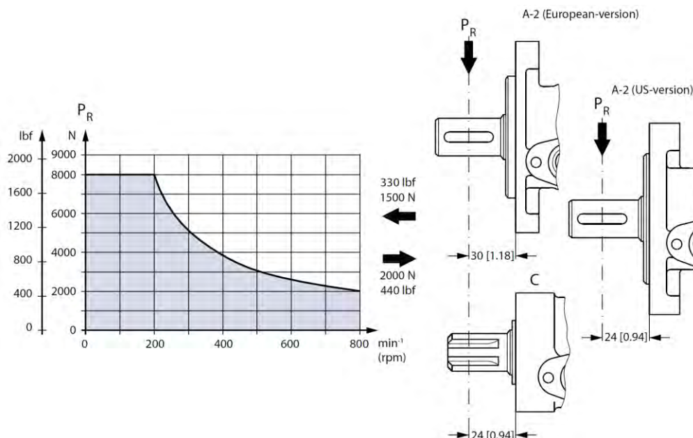
Figure 8 OMP X and OMR X shaft loads
