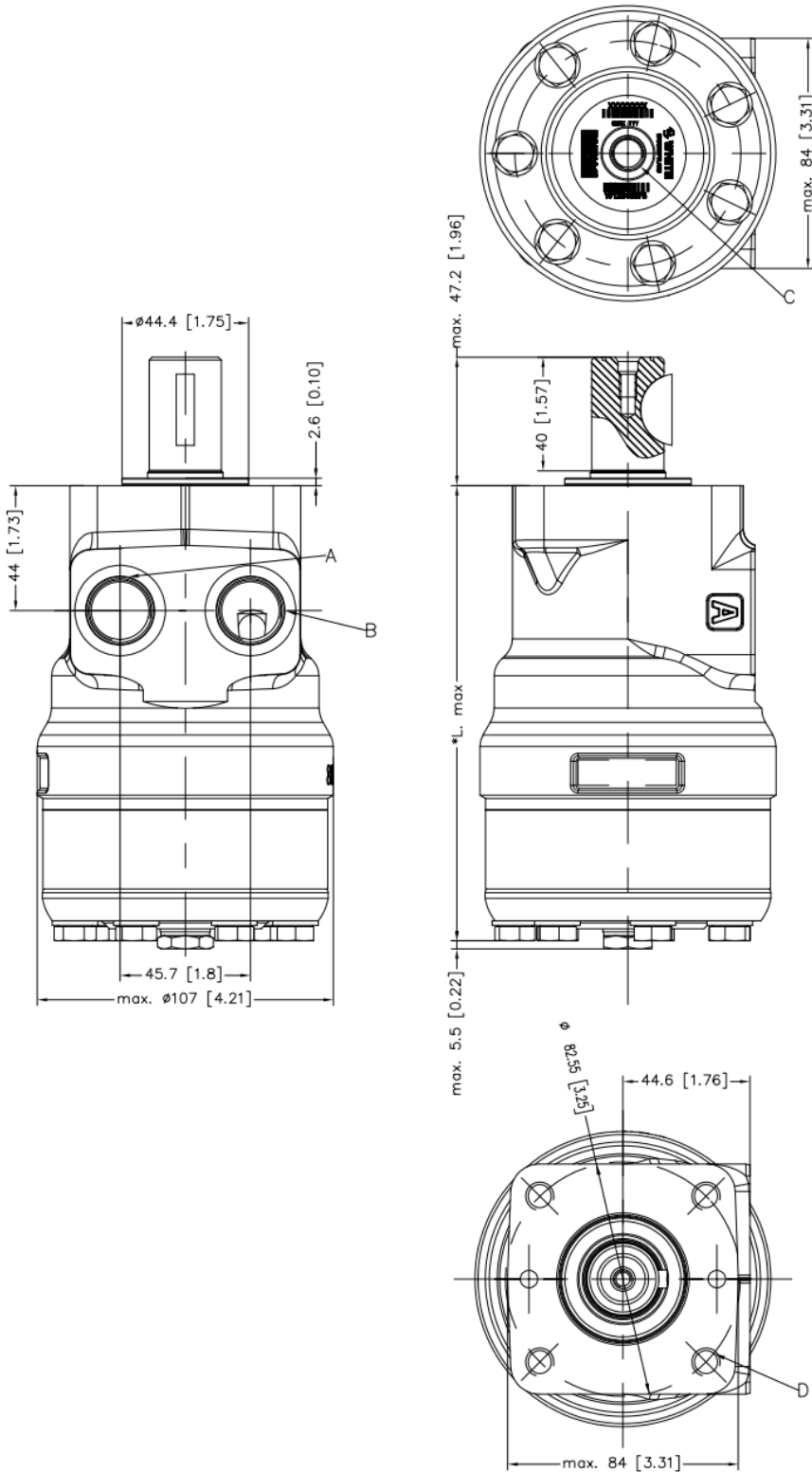
Figure 52 OMR X side port (C-flange) US version
