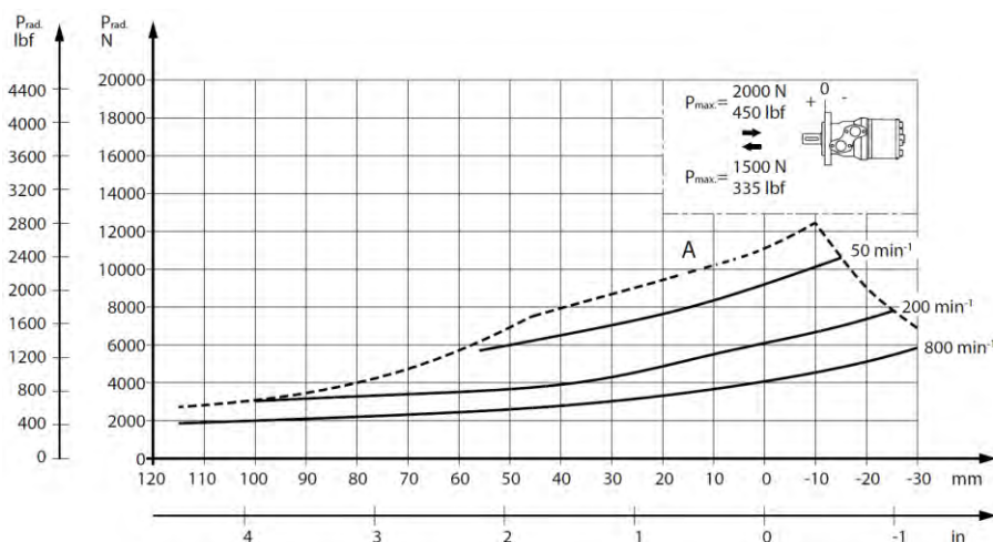
Figure 9 OMP X N shaft loads
