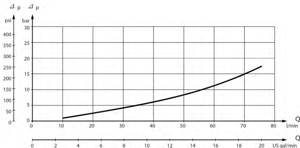
Figure 36 OMR X pressure drop
