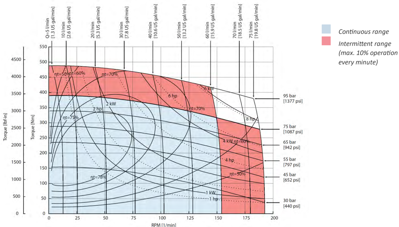
Figure 23 OMP X 400 function diagram
