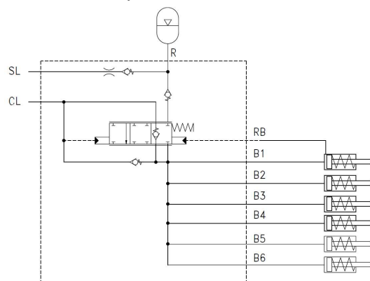
hydraulic schematic
