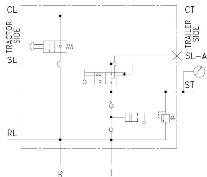
hydraulic schematic
