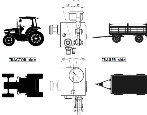
assembly position
