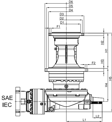
SELF PROPELLED MIXER DRIVE A2 PTO INPUT
