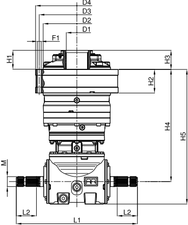
OUTPUT FLANGE INTERFACE
