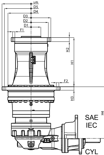
STATIONARY MIXER DRIVE A3 SAE/IEC/CYL INPUT
